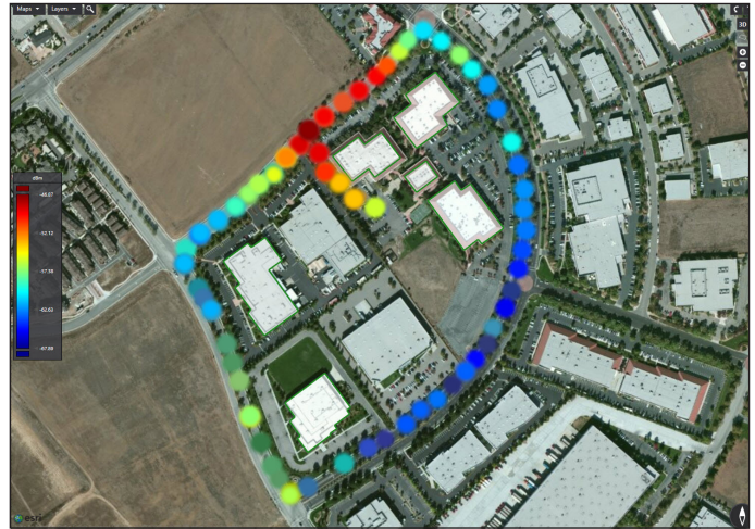
Typical result screen for outdoor coverage mapping
